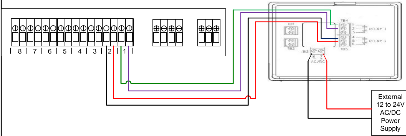
Figure 1.1: F200 Wiring
