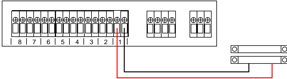
Figure 4.1: F200 Wiring
