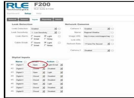
Figure 3.2: F200 Input Configuration Interface
