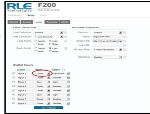
Figure 5-2: F200 Input Configuration Interface
