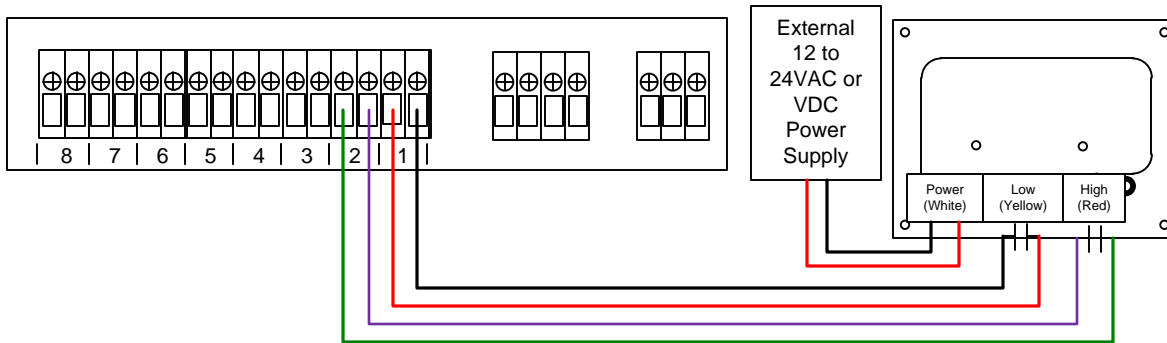
Figure 6.1: F200 Wiring
