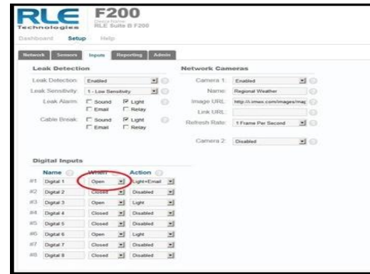
Figure 2.2 F200 Input Configuration
