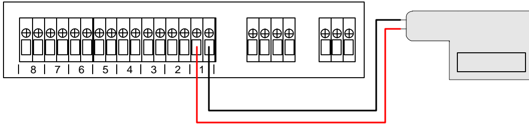
Figure 2.1: F200 Wiring
