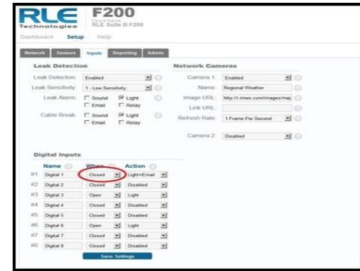
Figure 1.2: F200 Input Configuration Interface
