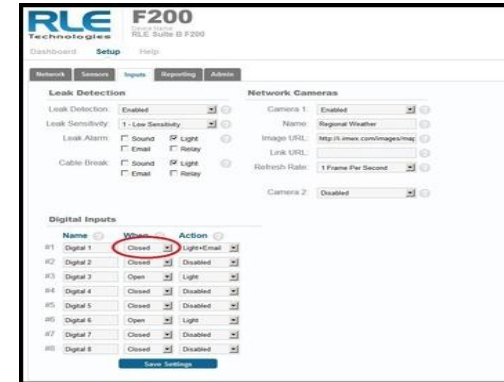
Figure 6.2: F200 Input Configuration Interface
