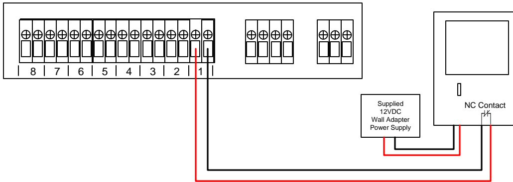
Figure 3.1: F200 Wiring
