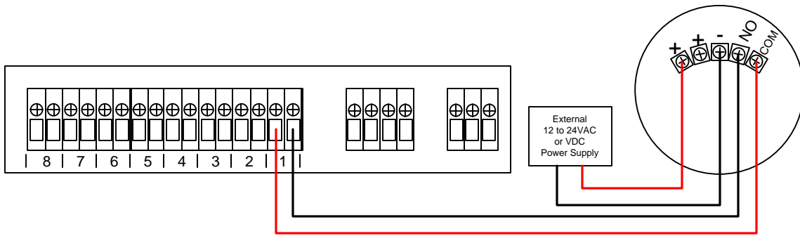
Figure 5.1: F200 Wiring
